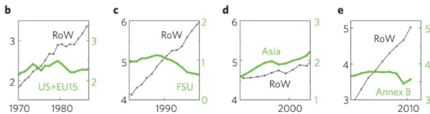
a , Emissions of CO 2 from fossil-fuel combustion and cement production for the world (Pg C yr -1 ; black curve) and the carbon intensity of world GDP (g C per $US (2000); red curve, inverted axis). The most important recent financial crises are highlighted with a linear trend fitted to the five years before the beginning of each crisis. b–e CO 2 emissions (Pg C) for the regions most affected by each financial crisis (right axis) and the rest of the world (RoW; left axis). b , The oil crisis (1973) and the US savings and loans crisis (1979), where EU15 is the 15 member states of the European Union as of 1995. c , The collapse of the Former Soviet Union (FSU; 1989). d , The Asian financial crisis (1997). e , The recent global financial crisis (2008–2009).
